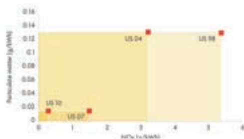
Figure 3. Tightening particulate matter and NO x limits.
