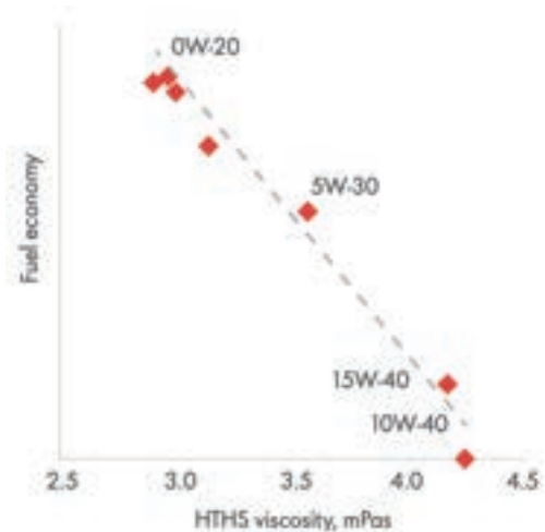
Figure 2. The relationship between HTHS viscosity and fuel economy.
